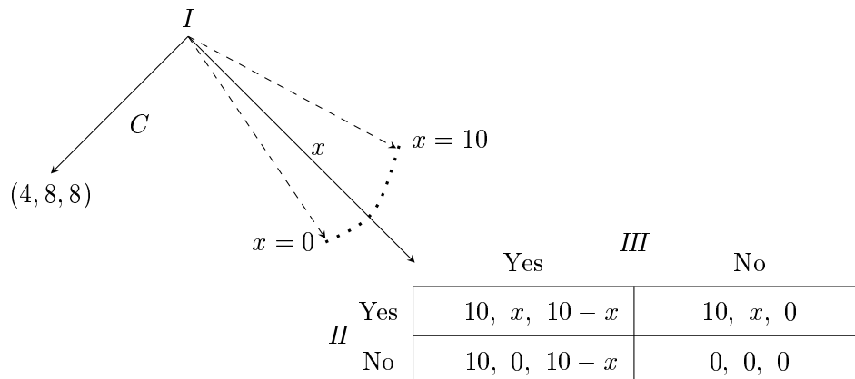
Figure 3: The extensive-form game \Gamma_2 . The choice x for player I ranges over the nonnegative integers, \{0, 1, \dots, 10\} .
