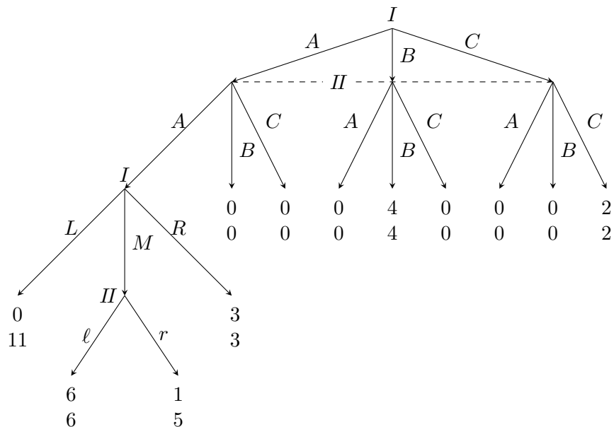
Figure 1: The game \Gamma_1 .
